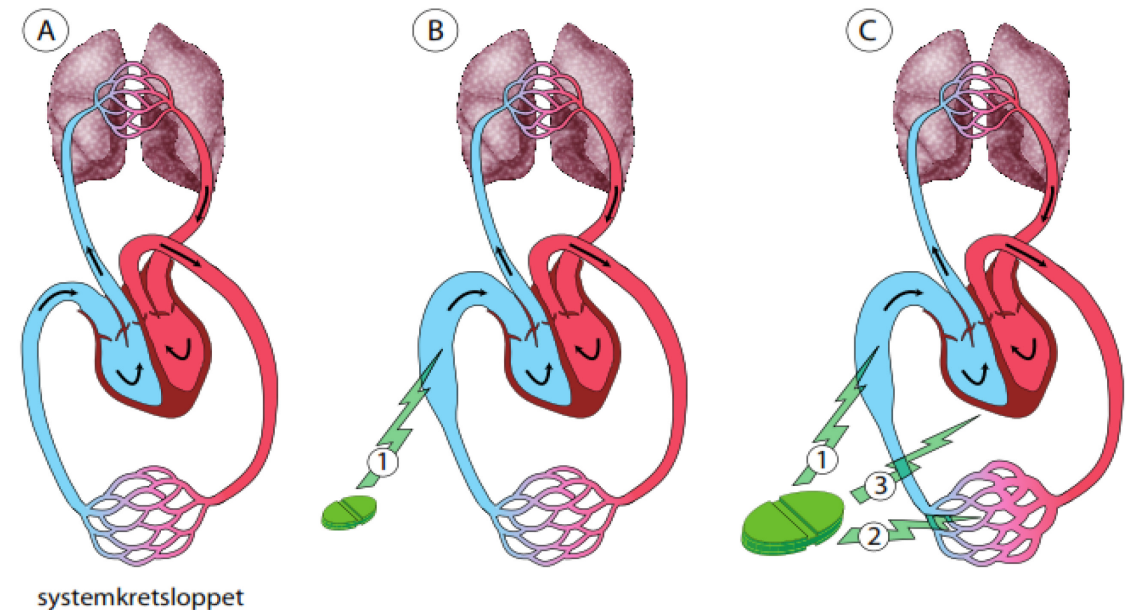
Figur 7.25 Organiska nitrater
